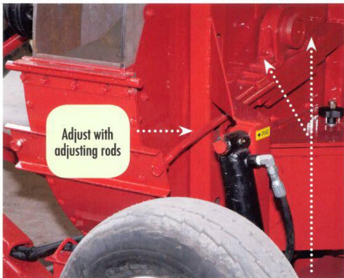
Blower paddle gap is easily adjusted by loosening 4 bearing bolts.
